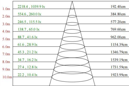
Max , Ave Beam angle of C112.5 plane 87.78
