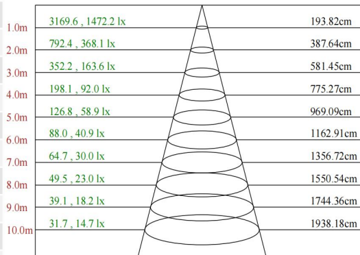
Max , Ave Beam angle of C112.5 plane 88.20
